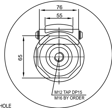
WIM(T)- 800S TYPE
